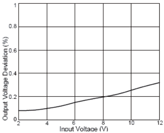
Fig.4 Line Regulation
